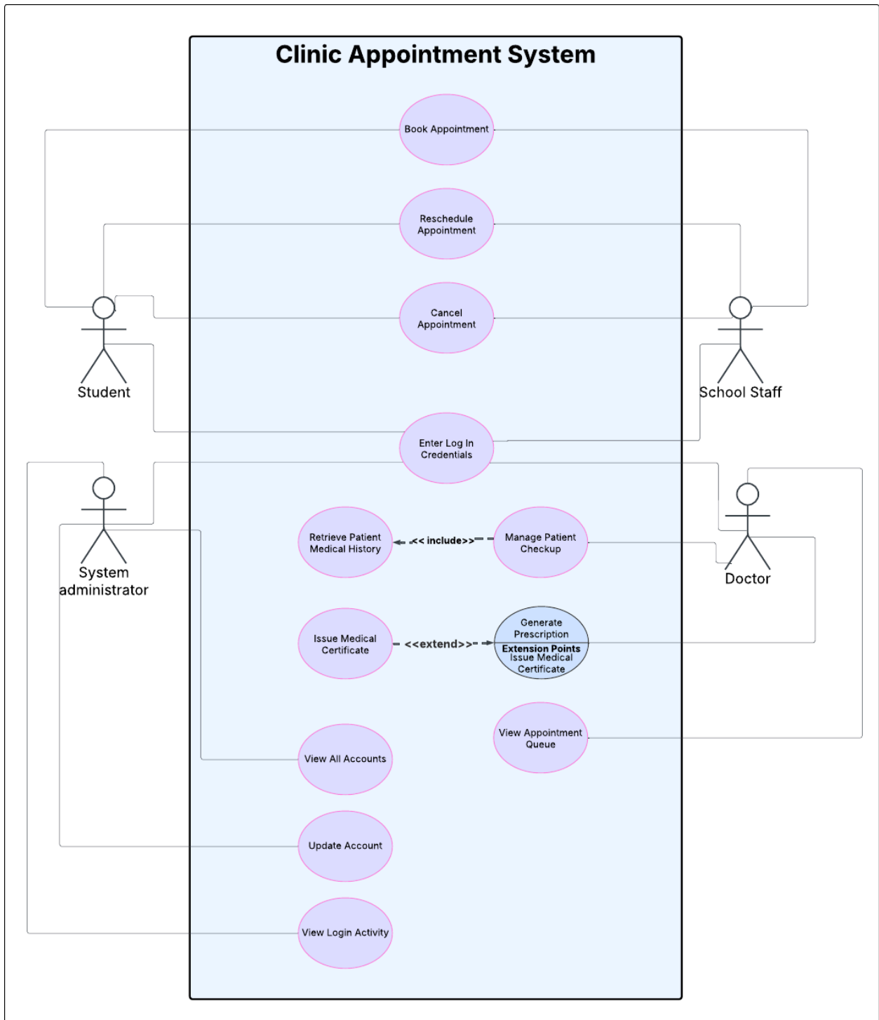
CLINIC APPOINTMENT SYSTEM USE CASE DIAGRAM
