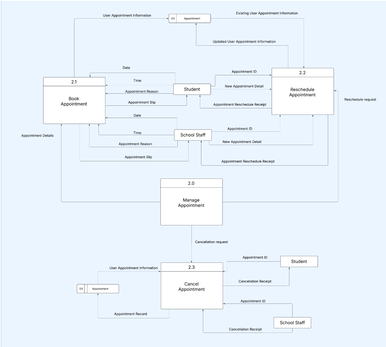
APPOINTMENT PROCESSES TLD
