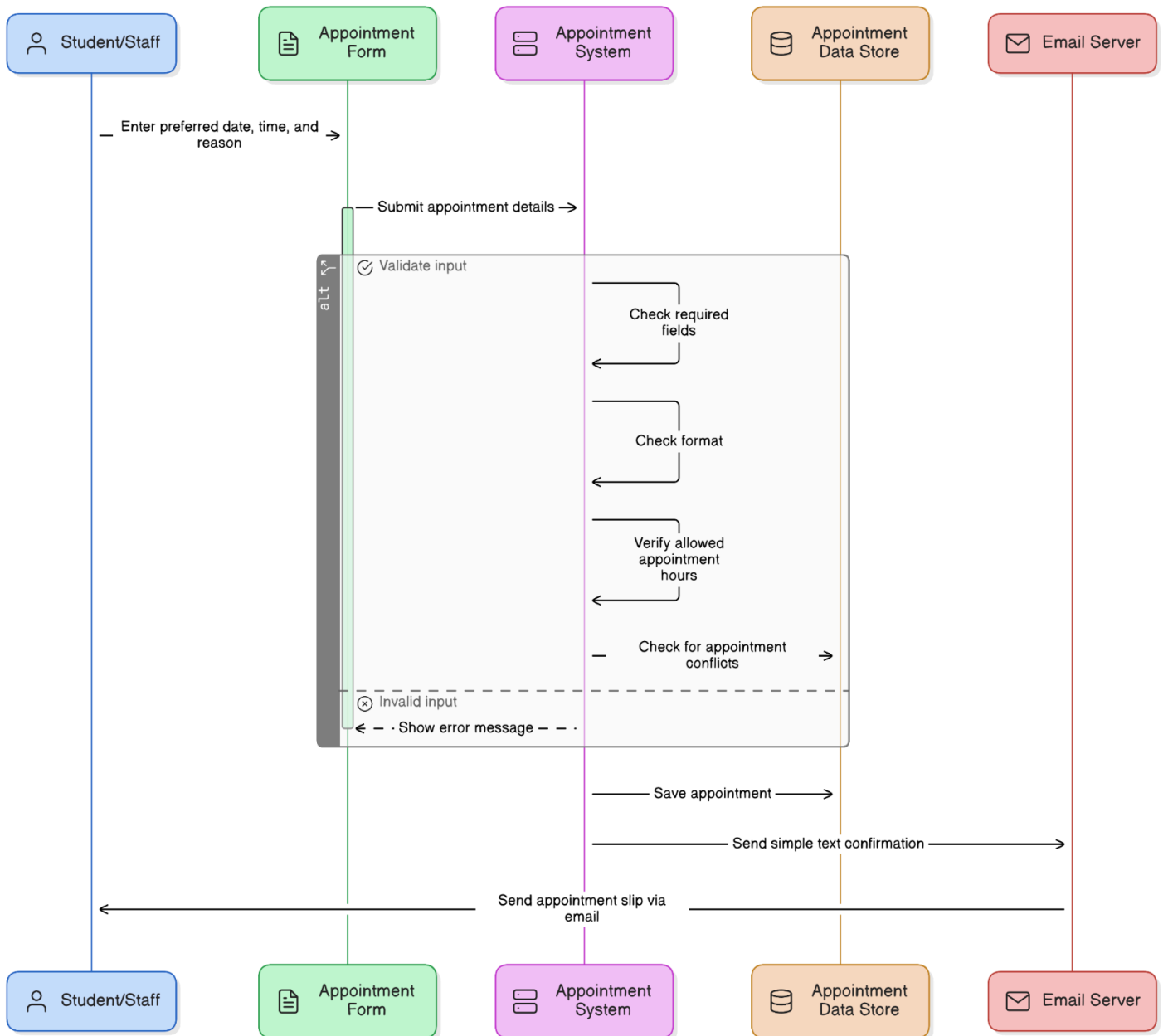
BOOK APPOINTMENT SEQUENCE DIAGRAM
