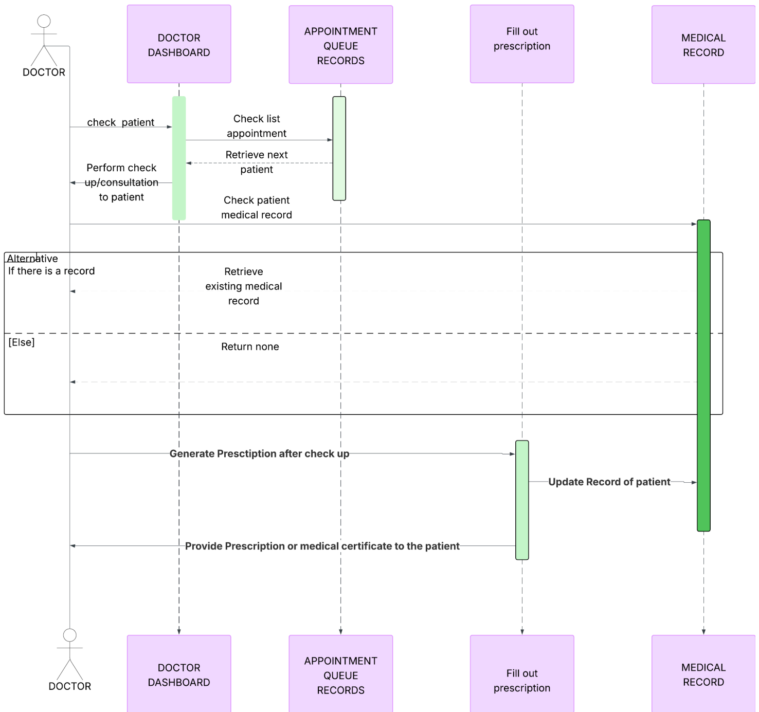
CHECK-UP PROCESS SEQUENCE DIAGRAM
